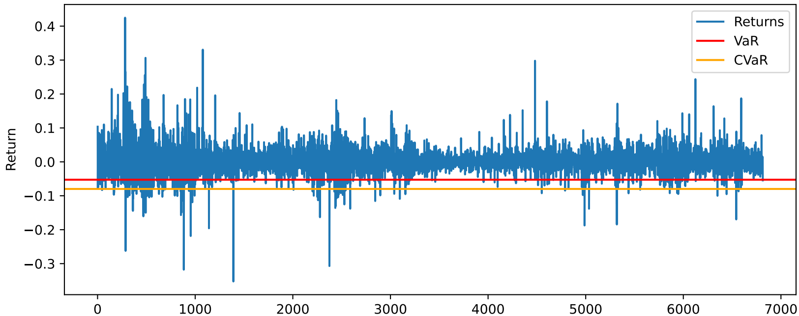
Returns, VaR, CVaR
